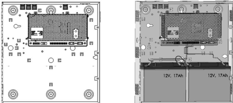
Figure 1 – E Box and Battery mounting
